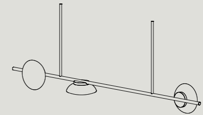
CH23L* L 1706MM W 200MM H 200MM^ L 67.2" W 7.9" H 7.9"^^ CEILING CANOPY SPACING L 840MM / 33.07"
