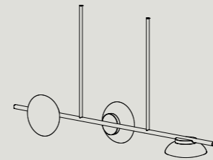
CH23S* L 1306MM W 200MM H 200MM^ L 51.4" W 7.9" H 7.9"^^ CEILING CANOPY SPACING L 440MM / 17.32"
