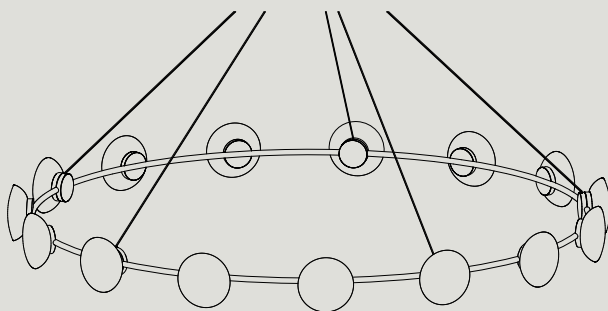
CC2015 Ø 2175 H 200 RING Ø 2000 Ø 7'2" H 7.9" RING Ø 6' 7" MIN DROP HEIGHT - H 1200 / 3'11"
